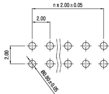
PCB Layouts
